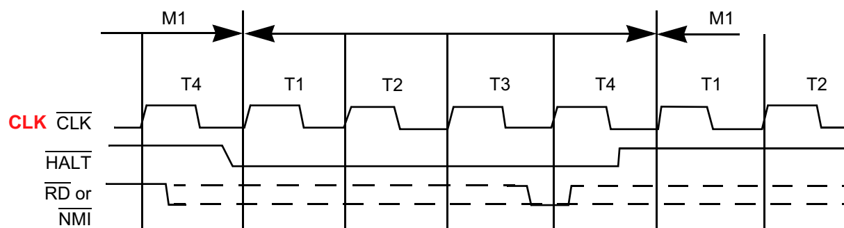
Figure 11. HALT Exit
