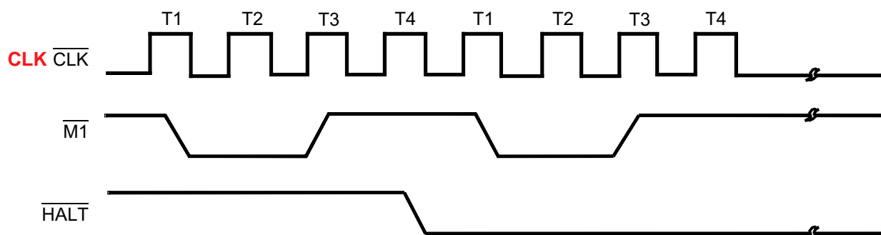
Figure 12. Power-Down Acknowledge
