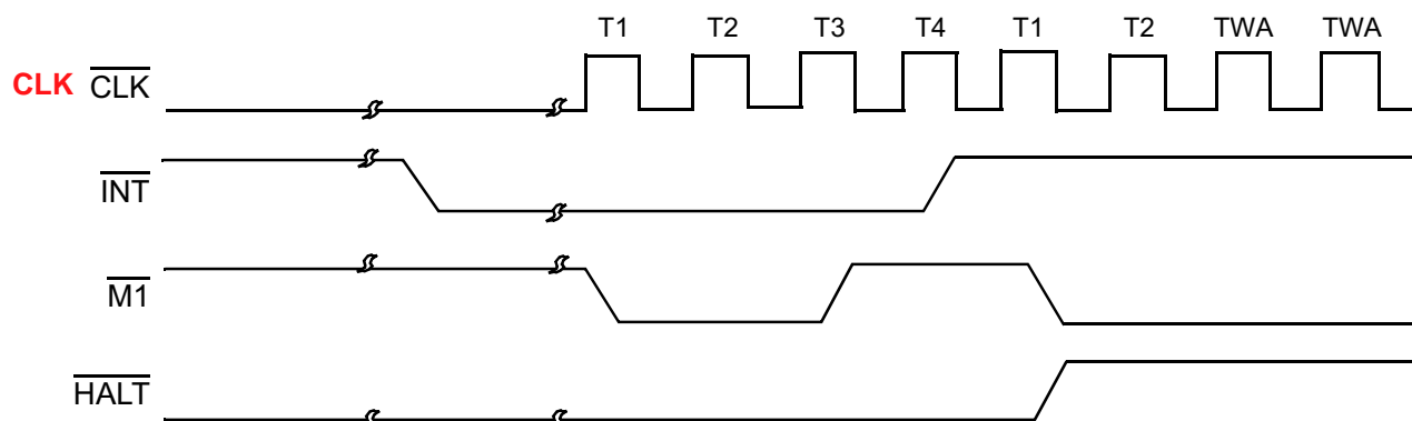
Figure 15. Power-Down Release Cycle, #3 of 3
