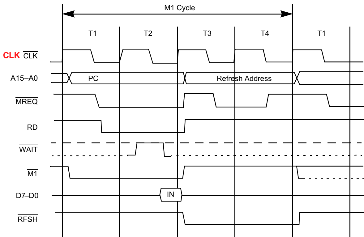
Figure 5. Instruction Op Code Fetch
