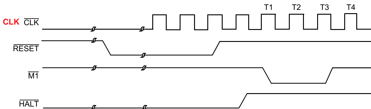
Figure 14. Power-Down Release Cycle, #2 of 3
