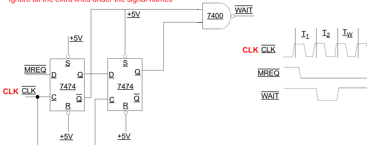
Figure 22. Adding One Wait State to Any Memory Cycle
